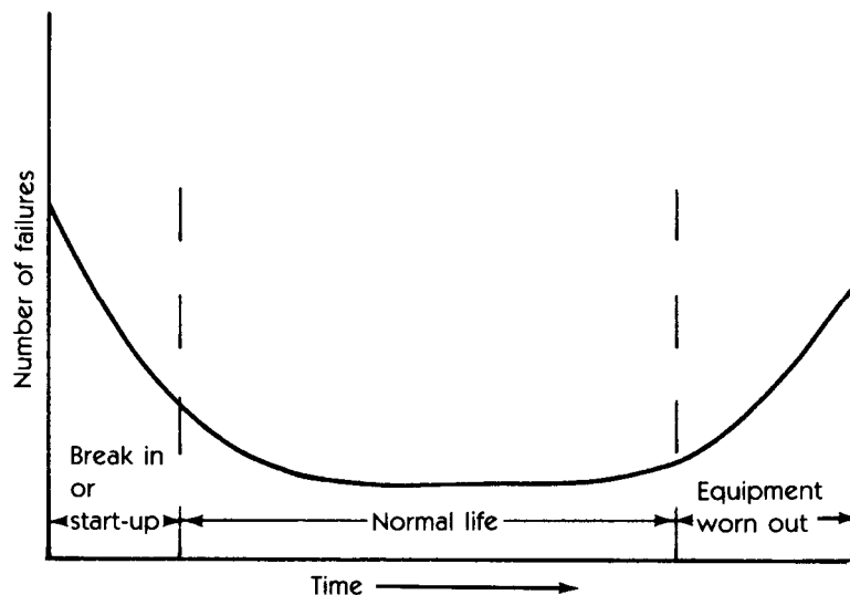
Figure 1. Bathtub Curve
